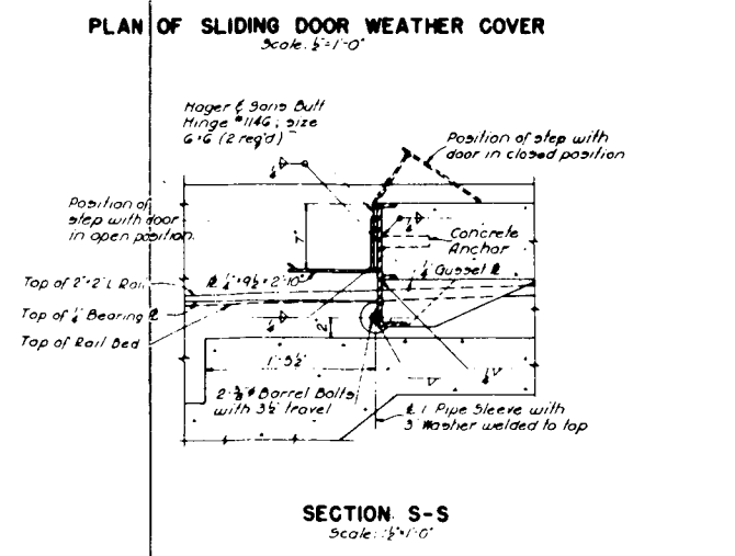
Fig. 17—Entrance details, underground personnel shelter.
